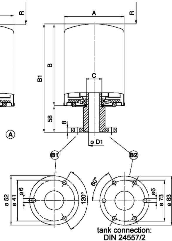
Dwg. B Flanged connector
