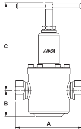
1 1/2" to 2" – DN 40 to DN 50
