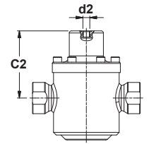
Optional dome-loaded version
