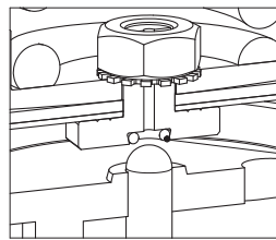
Optional relieving version
