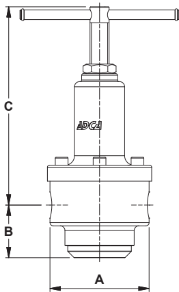
1" to 1 1/4" – DN 25 to DN 32
